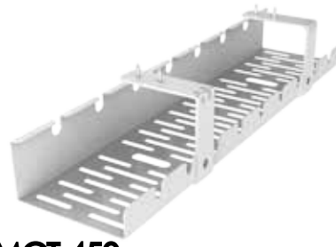
MCT 450 Mesh cable tray (500w x 122d x 90h )
